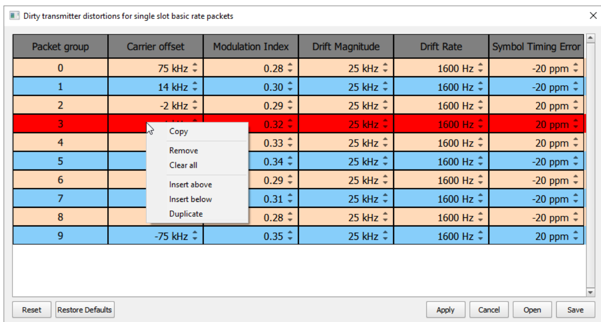
Figure 5: Dirty transmitter dialogue box displaying the waveform distortion table currently in use.
