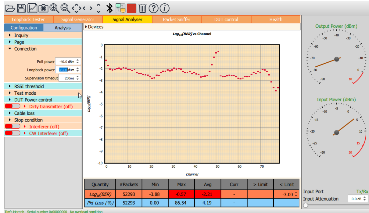
Figure 30: Adjusting the signal level during receiver testing
