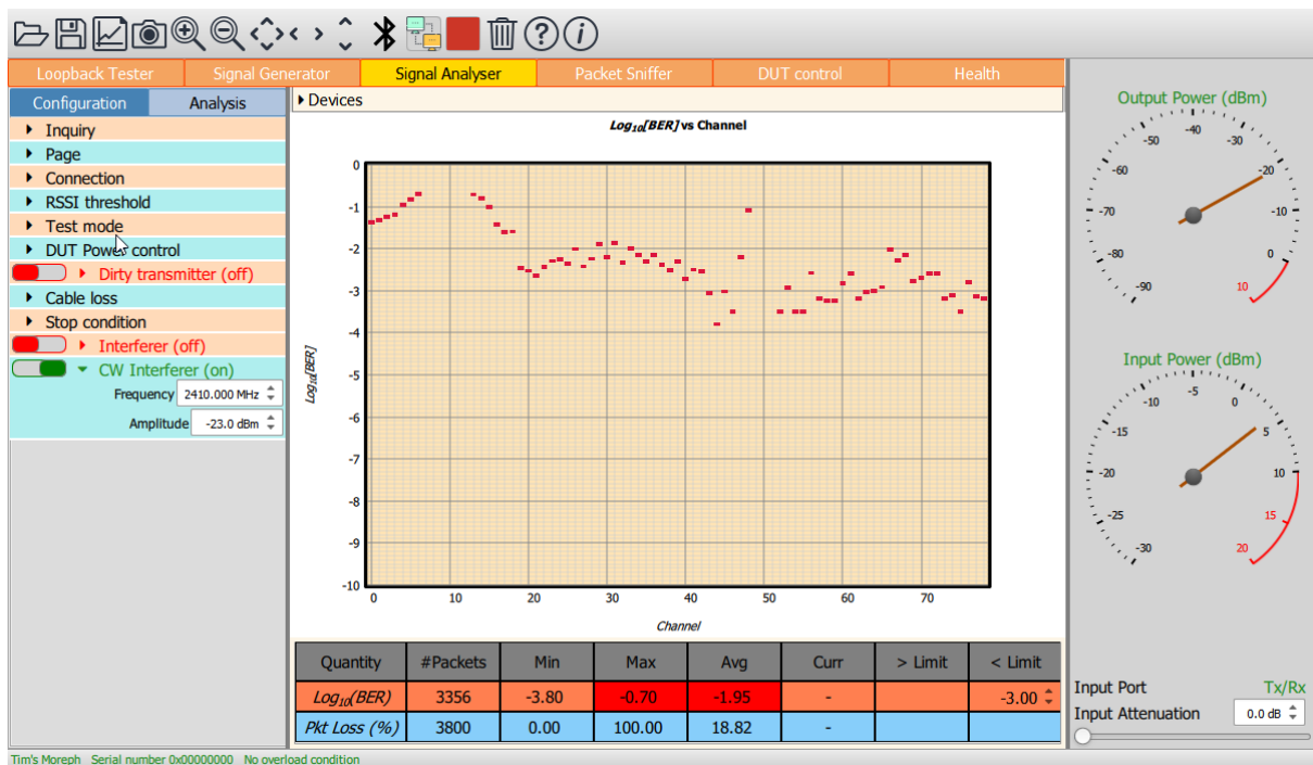
Figure 32: Adding a modulated interferer during receiver testing
