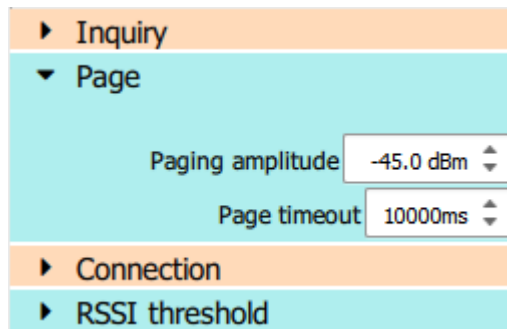
Figure 78: Controlling paging
