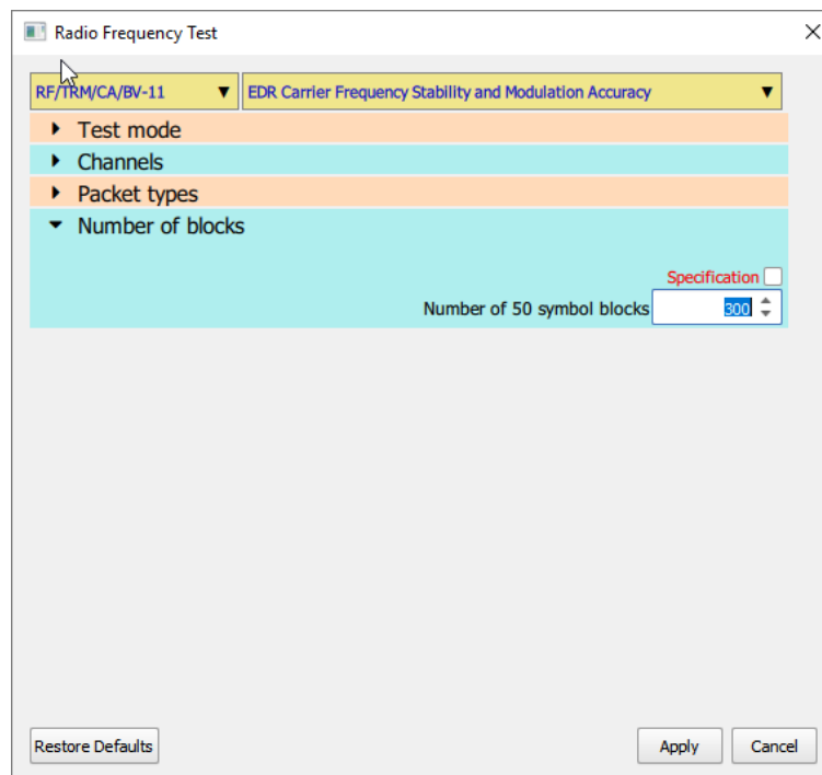
Figure 45: Selecting the number of 50 symbol blocks for the EDR carrier frequency stability and modulation accuracy test (RF/TRM/CA/BV-11-C).
