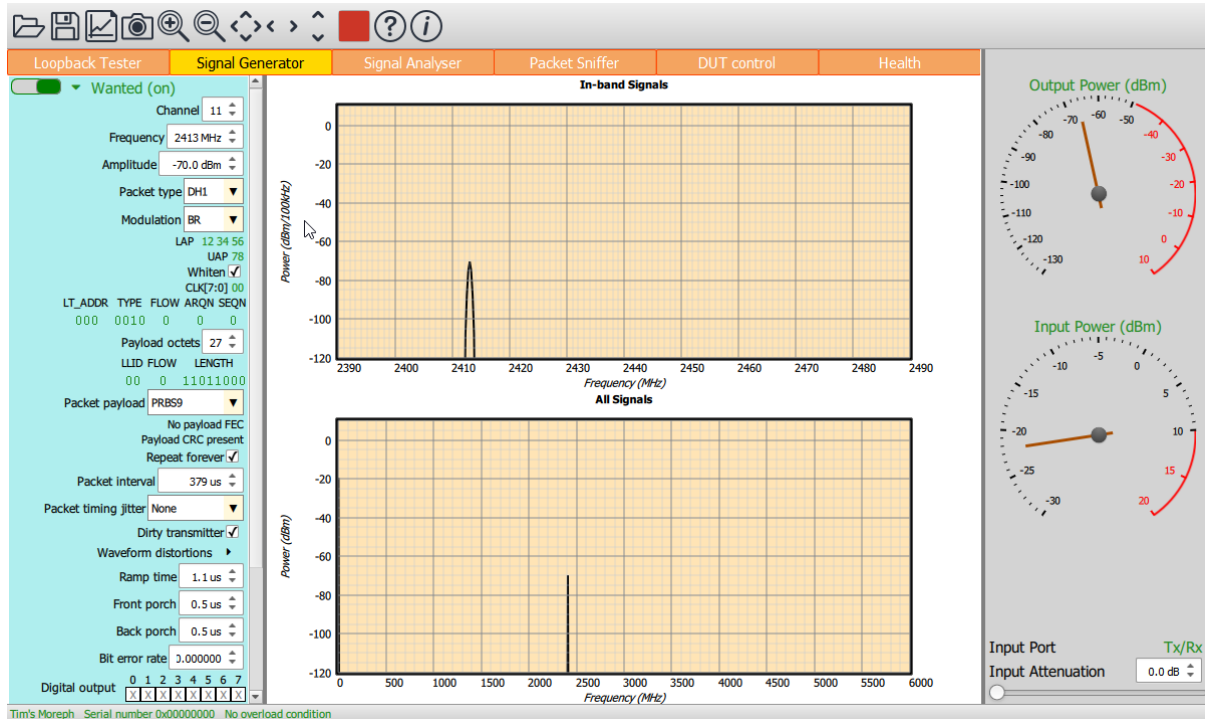
Figure 4: Programming the packetised BR/EDR signal.
