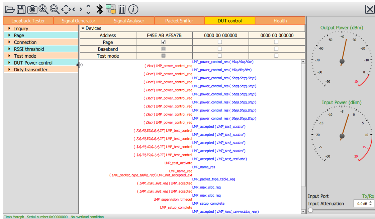
Figure 74: DUT control mode
