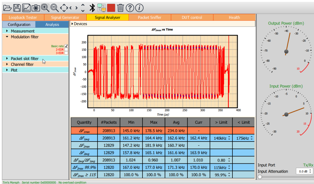
Figure 15: Filtering displayed results by modulation.
