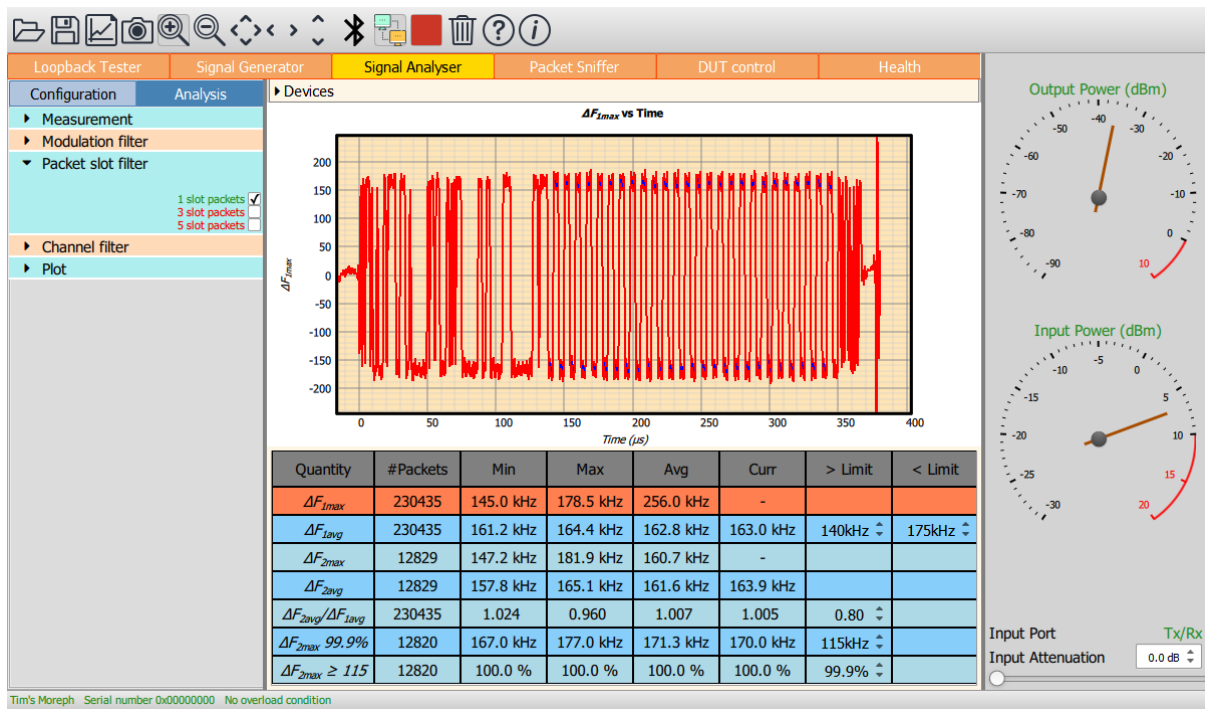
Figure 16: Filtering displayed result by packet slots.
