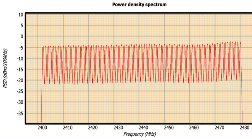
Figure 28: Power density spectrum.
