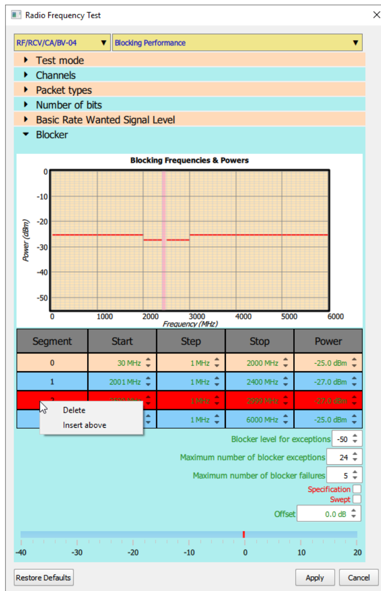
Figure 58: Removing or adding blocker frequencies and levels.
