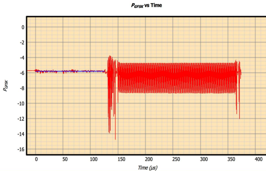
Figure 22: EDR power profile vs time.
