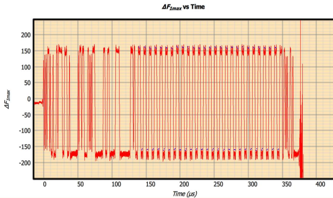
Figure 23: FM demodulated waveform vs time.
