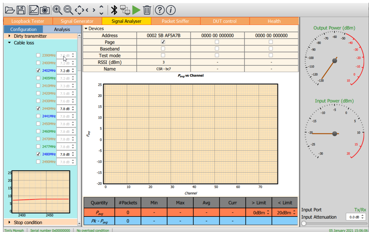
Figure 12: Programming the cable loss.
