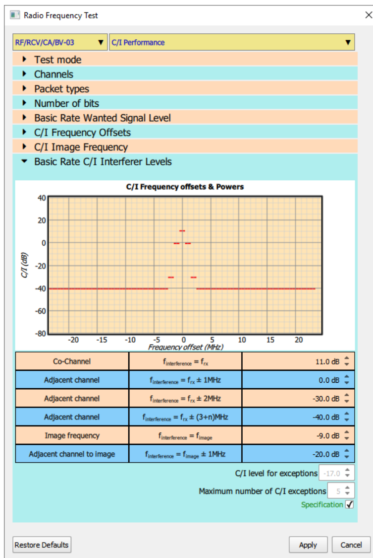
Figure 54: Interferer signal level for C/I receiver tests.
