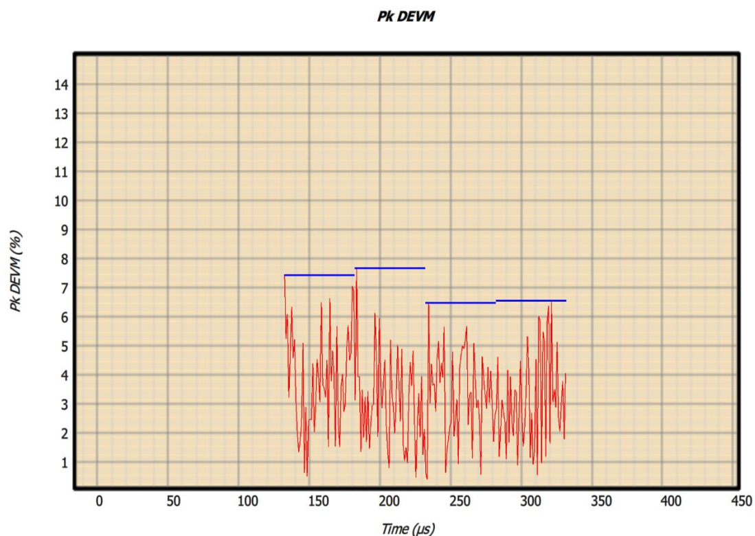
Figure 24: EDR DEVM profile vs time.
