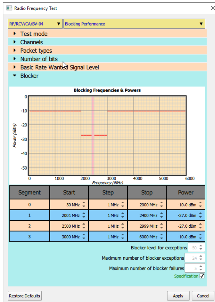
Figure 57: Blocker frequencies and levels.
