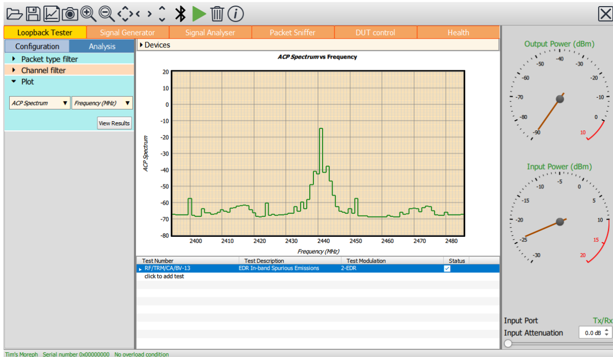
Figure 66: Example of additional data being displayed for EDR in-band spurious emissions test.
