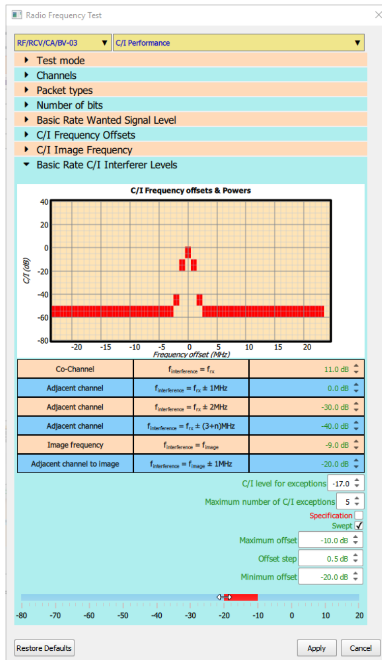
Figure 56: Selecting a range of signal levels for C/I receiver tests.
