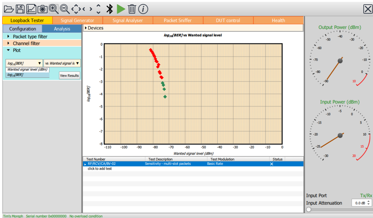
Figure 67: Receiver sensitivity test showing \text{Log}_{10}(\text{BER}) vs signal level
