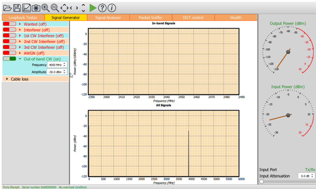
Figure 9: Programming the out-of-band CW interferer signal.
