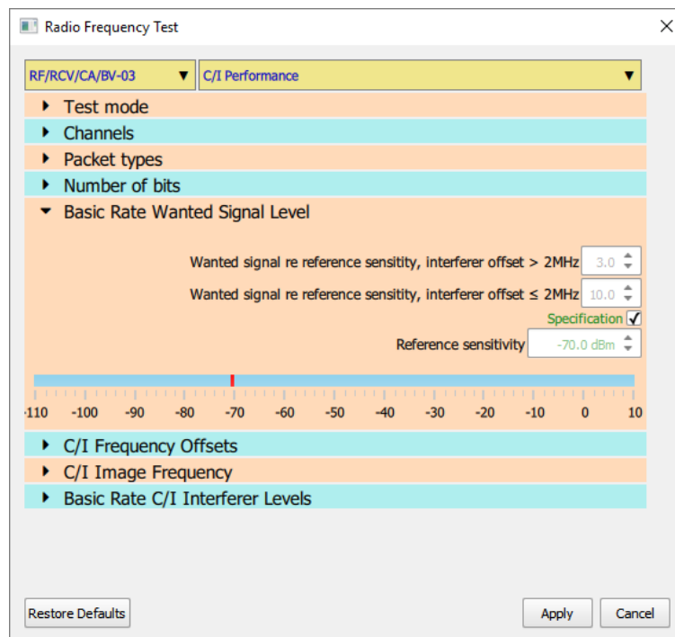
Figure 50: Entering the wanted signal level for C/I performance tests.
