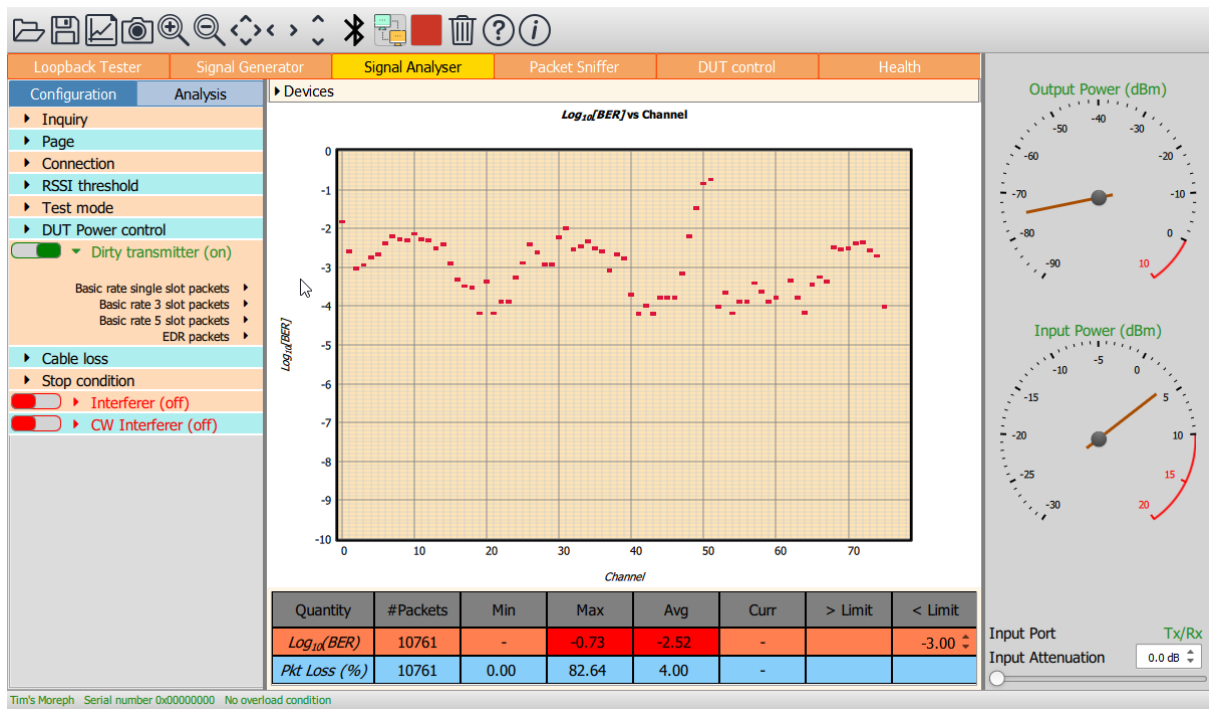
Figure 31: Turning on the dirty transmitter during receiver testing
