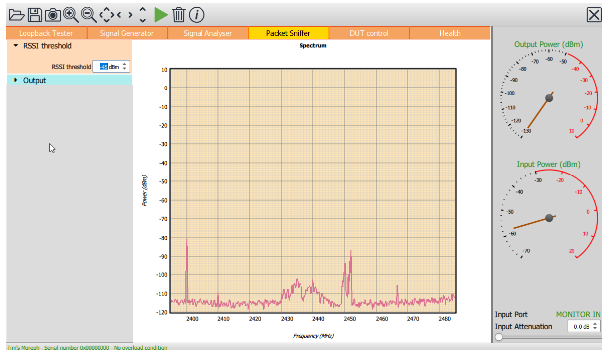
Figure 72: Programming the sniffer RSSI threshold.
