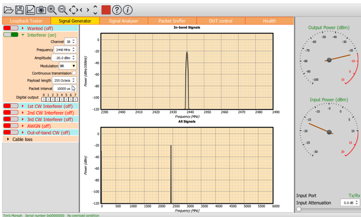
Figure 6: Programming the modulated interferer signal.
