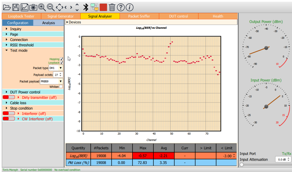
Figure 29: Example test mode suitable for performing receiver testing
