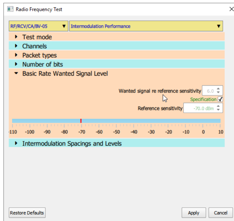
Figure 51: Entering the wanted signal level for blocking and intermodulation tests.
