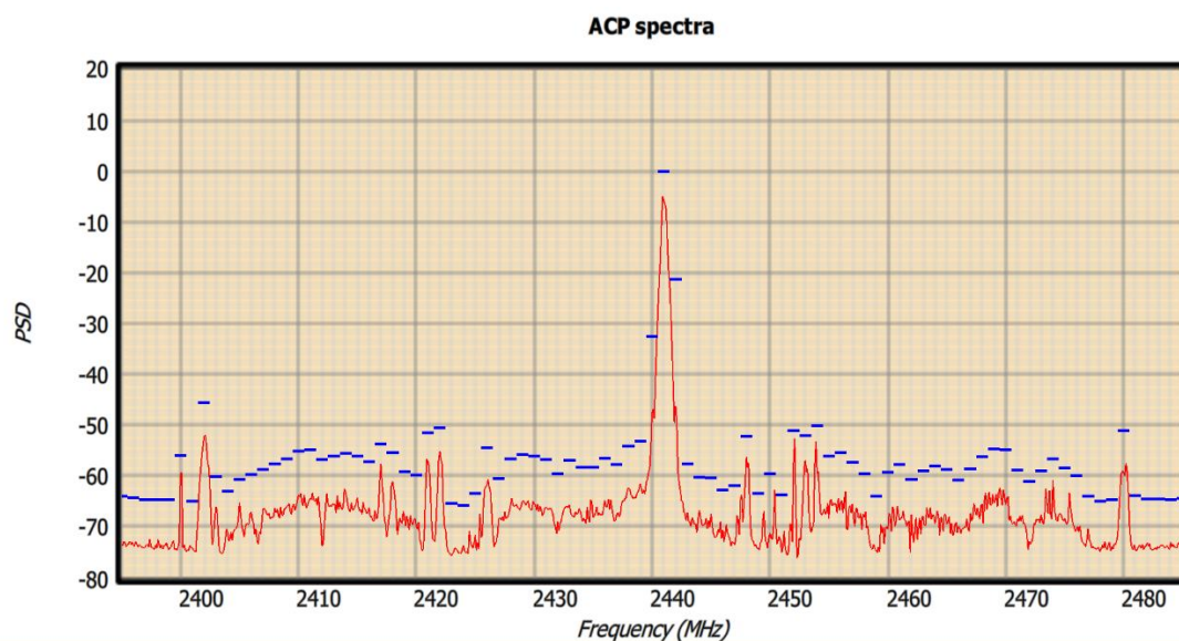
Figure 27: Adjacent power spectrum.
