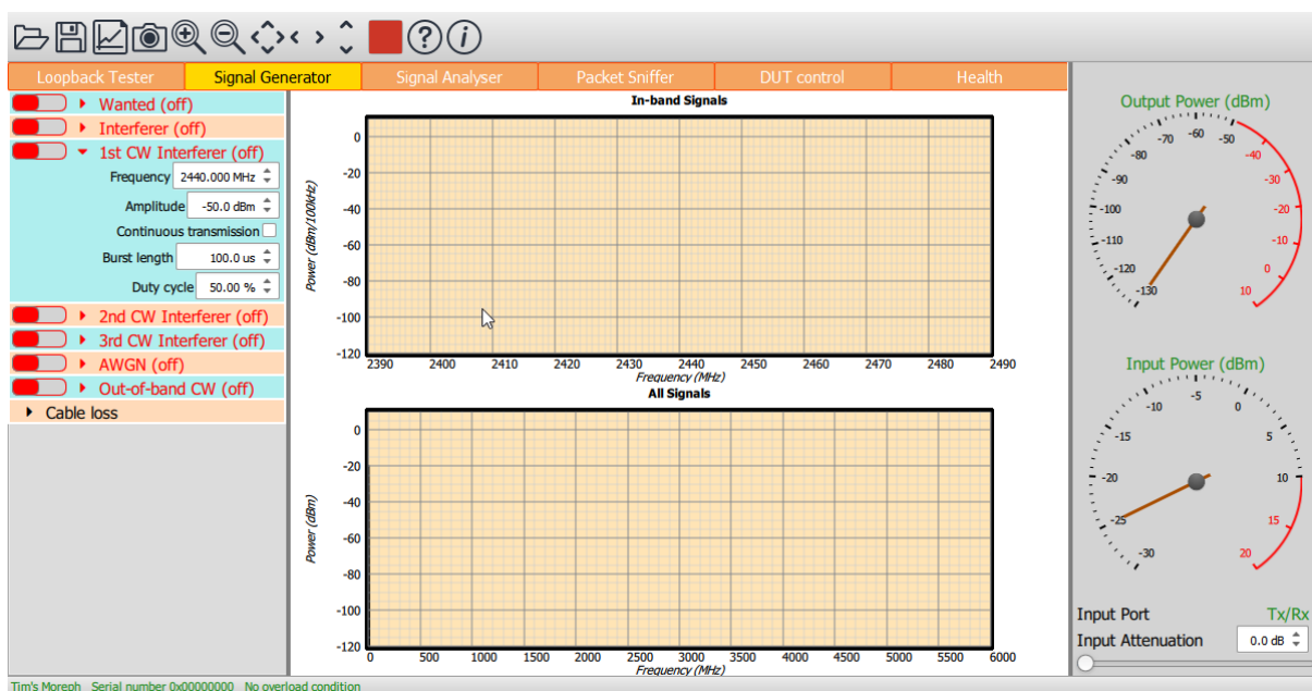
Figure 7: Programming an in-band CW interferer signal.
