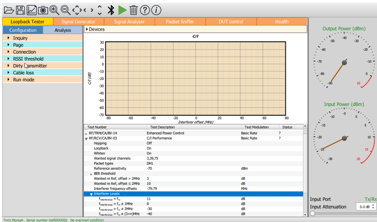
Figure 62: The test script window.
