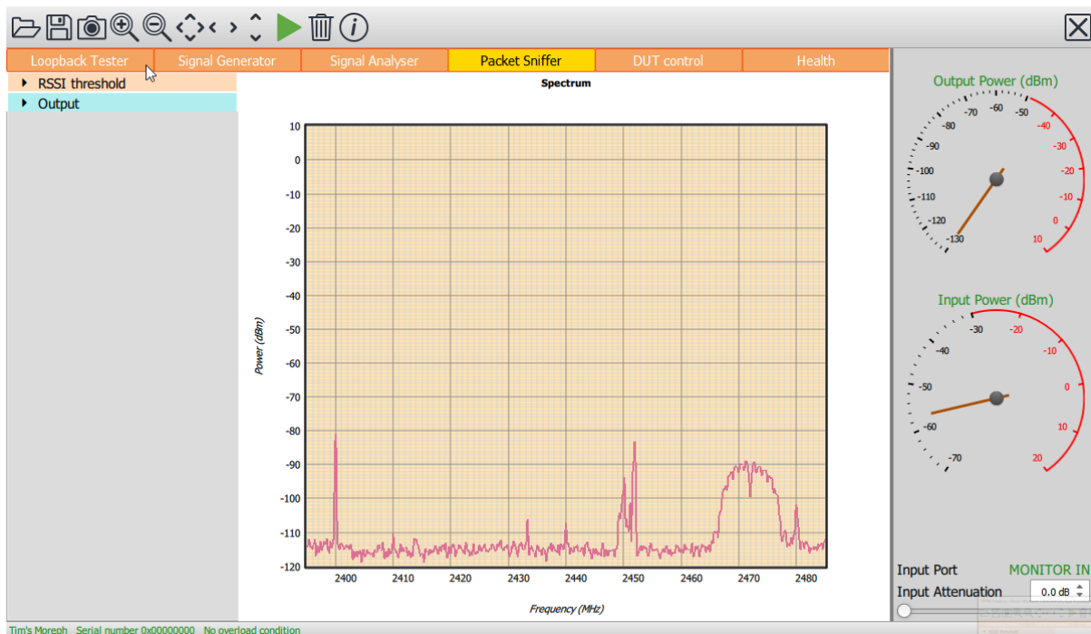
Figure 71: Zircon packet sniffer mode.
