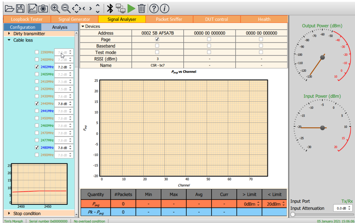
Figure 34: Entering the cable loss value.
