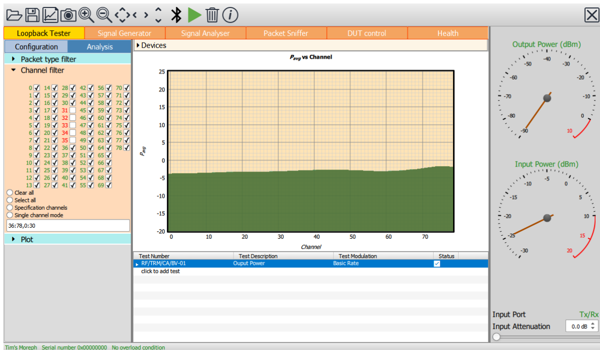
Figure 64: Filtering by RF channel.
