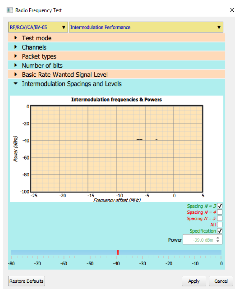
Figure 60: Configuring the intermodulation test.
