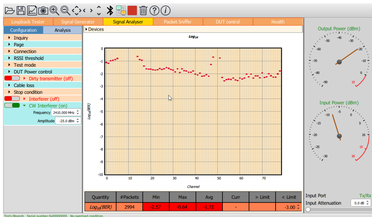
Figure 33: Adding a CW interferer during receiver testing
