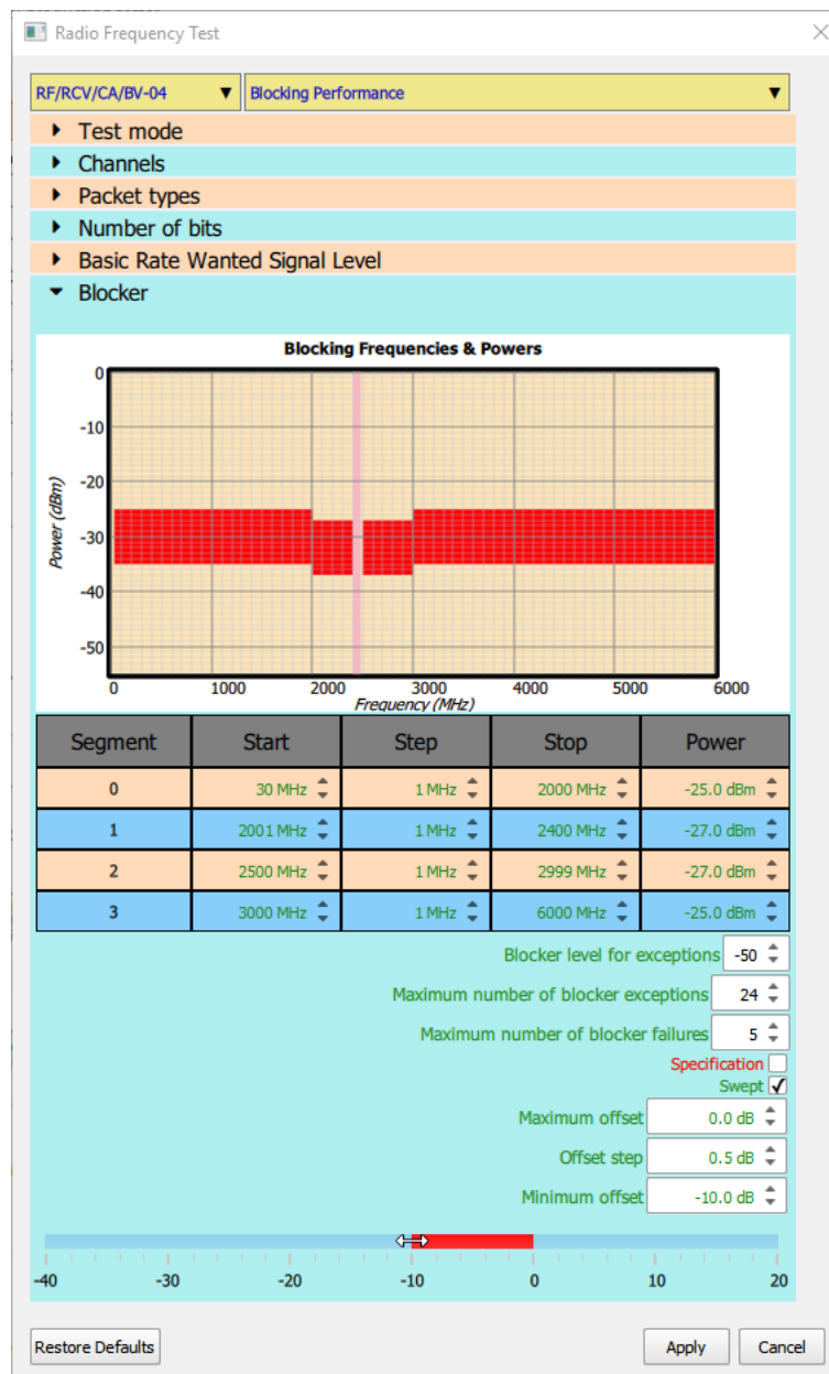
Figure 59: Selecting a range of blocker frequencies and levels.
