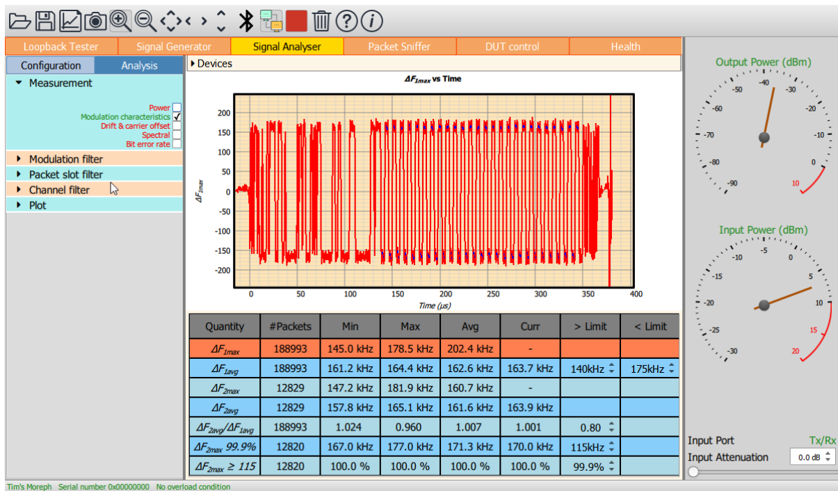
Figure 14: Selecting the measurement group to display.
