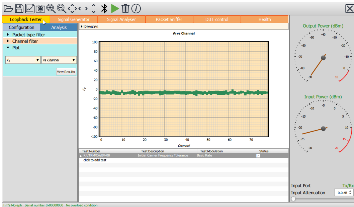
Figure 65: Example display of transmitter test vs channel.
