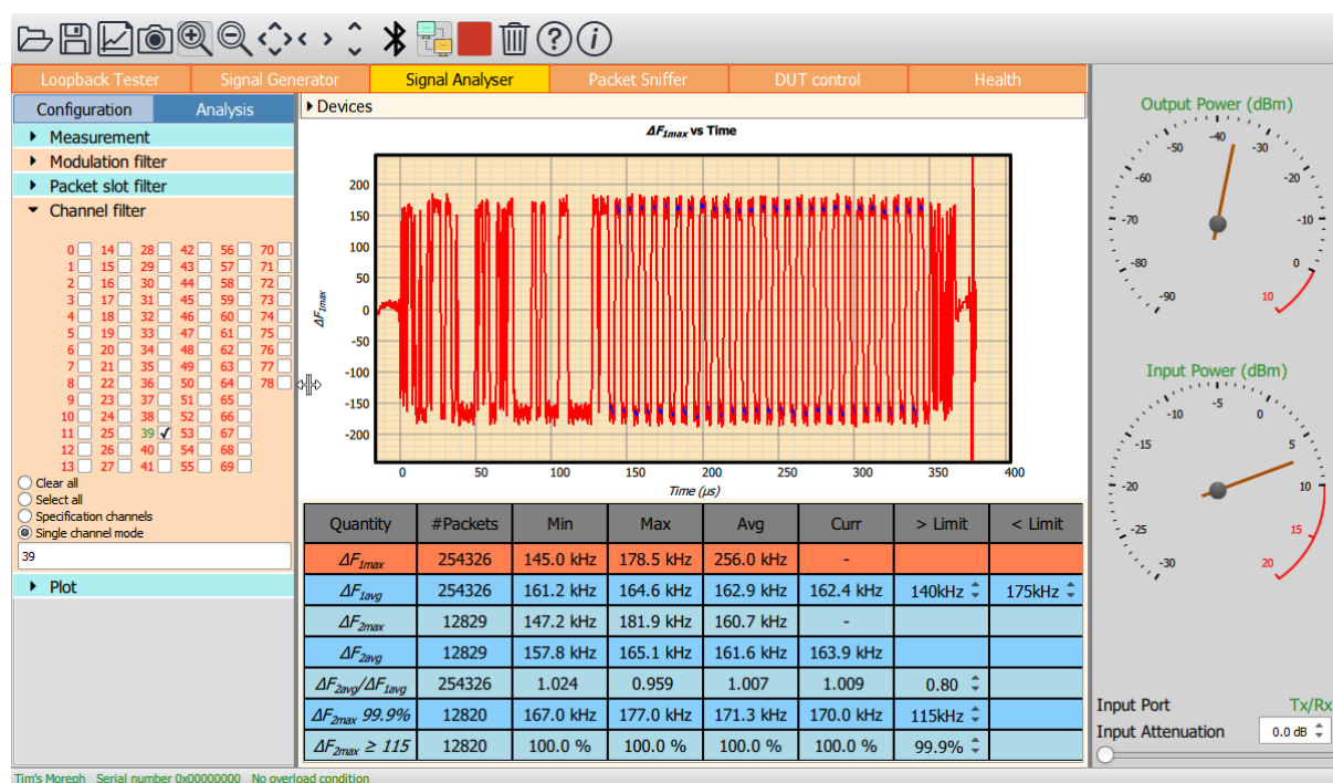
Figure 17: Filtering displayed results by RF channel.
