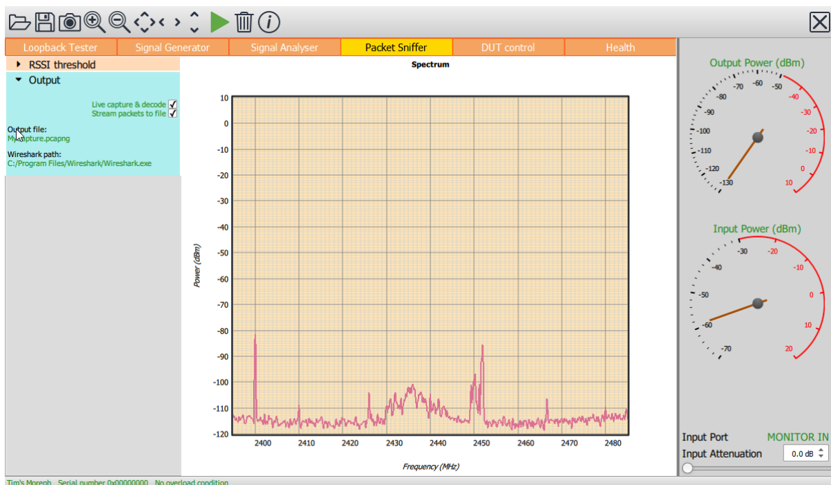
Figure 73: Programming the packet data sink
