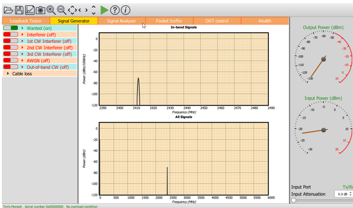
Figure 3: Zircon GUI in signal generator mode.
