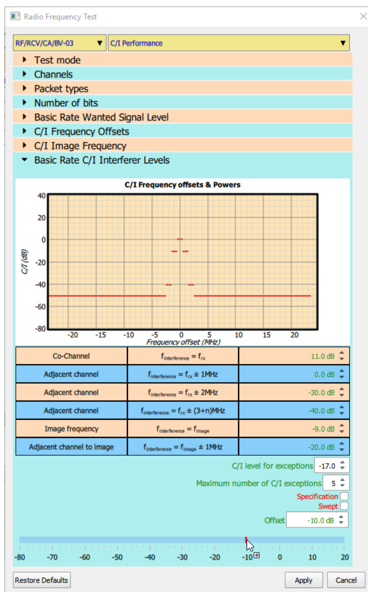
Figure 55: Changing the signal level for C/I receiver tests.
