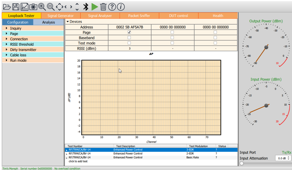
Figure 42: Test script resulting from adding enhanced power control test (RF/TRM/CA/BV-14-C).
